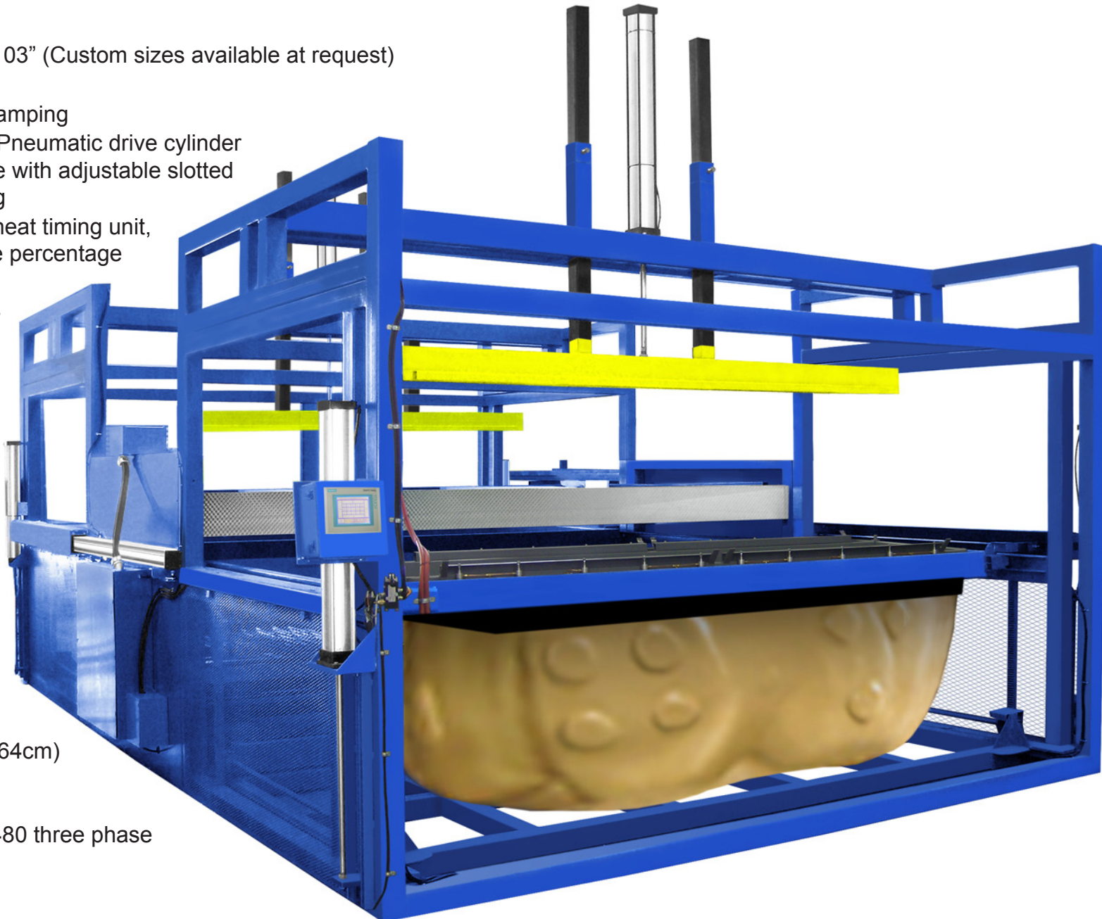
Model BV E-Class 53" x 33" or 53" x 53" Double-Ended Shuttle Vacuum Former
