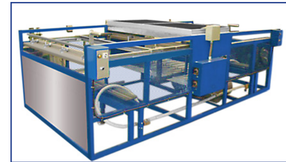
Model BV E-Class 53" x 33" or 53" x 53" Double-Ended Shuttle Vacuum Former
