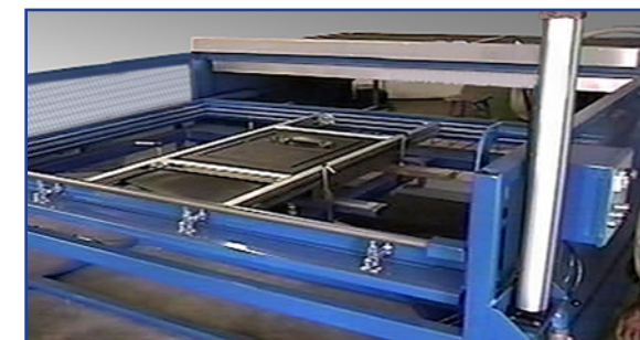
Adjustable Power Strut Plastic Clamping
